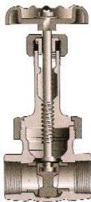
Fig. 88 RS Globe / Needle Style
